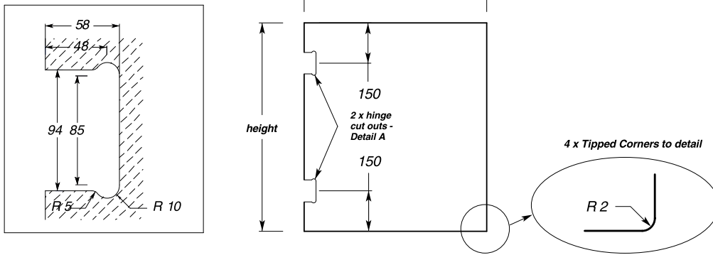
Detail A - Hinge cut out
