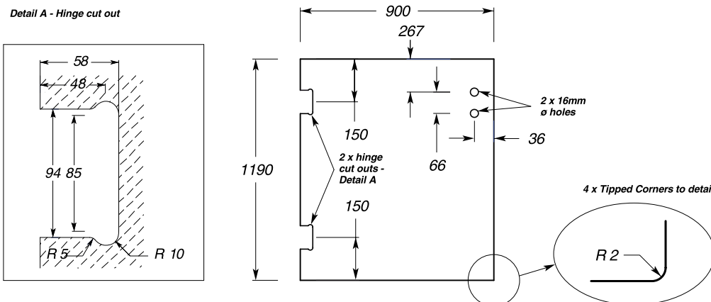
Detail A - Hinge cut out
