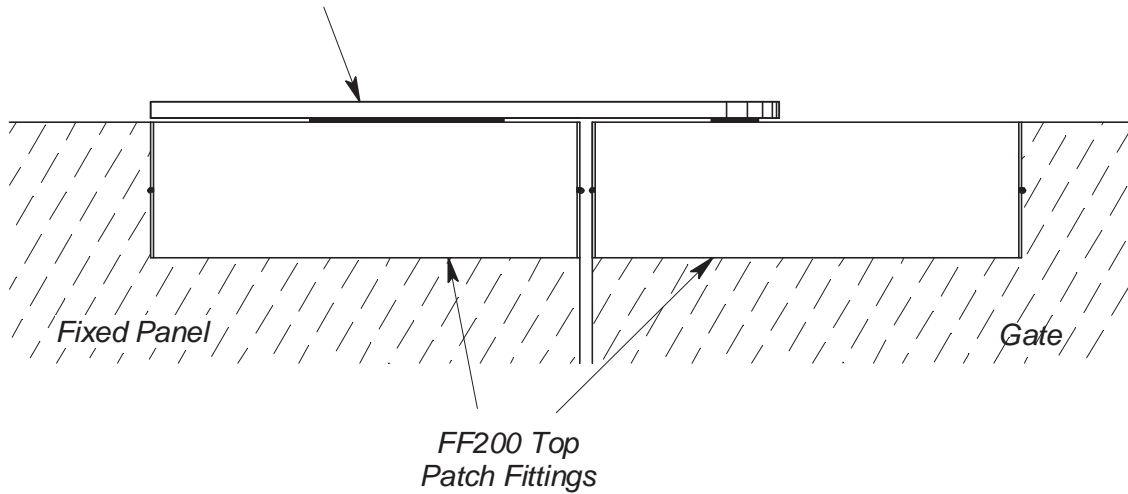
FPF7 Slimline Glass to Glass Pivot
